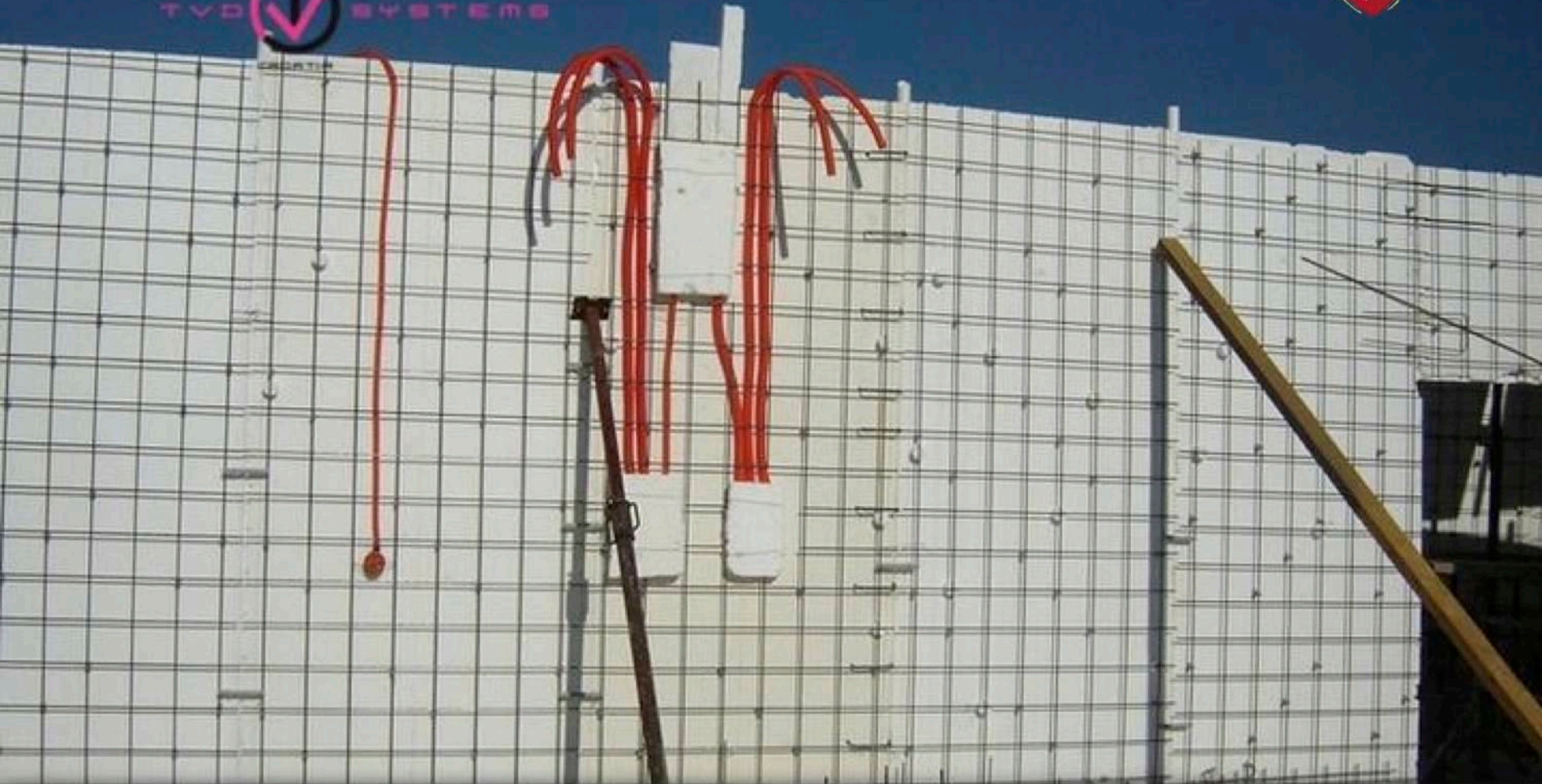
wall installation power line embedding
